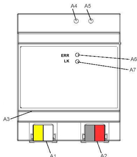
Figure 1: Location of the display and operating elements
